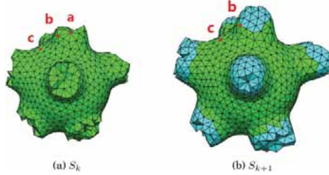
Fig. 4. Evolution of S_k to S_{k+1} . The UTC colored in green has a d_t \leq k , whereas the UTC with a d_t = k + 1 is colored in cyan.
